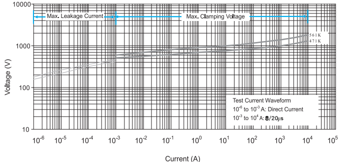
V-I Curve for SR471K~561K05D(E) Series
