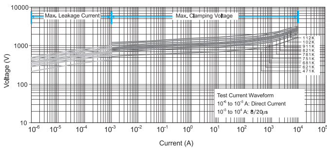
V-I Curve for SR471K~ 112K18E Series
