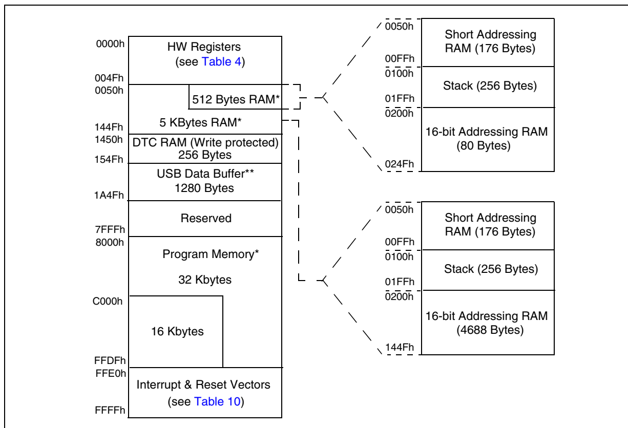
Figure 10. Memory Map
