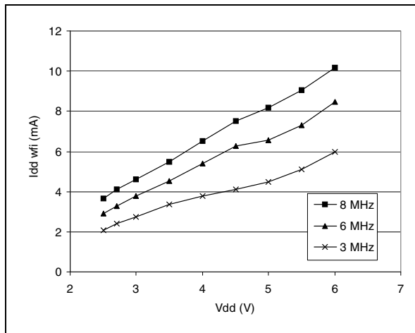
Figure 72. Typical I_{DD} in WAIT vs. f_{CPU}
