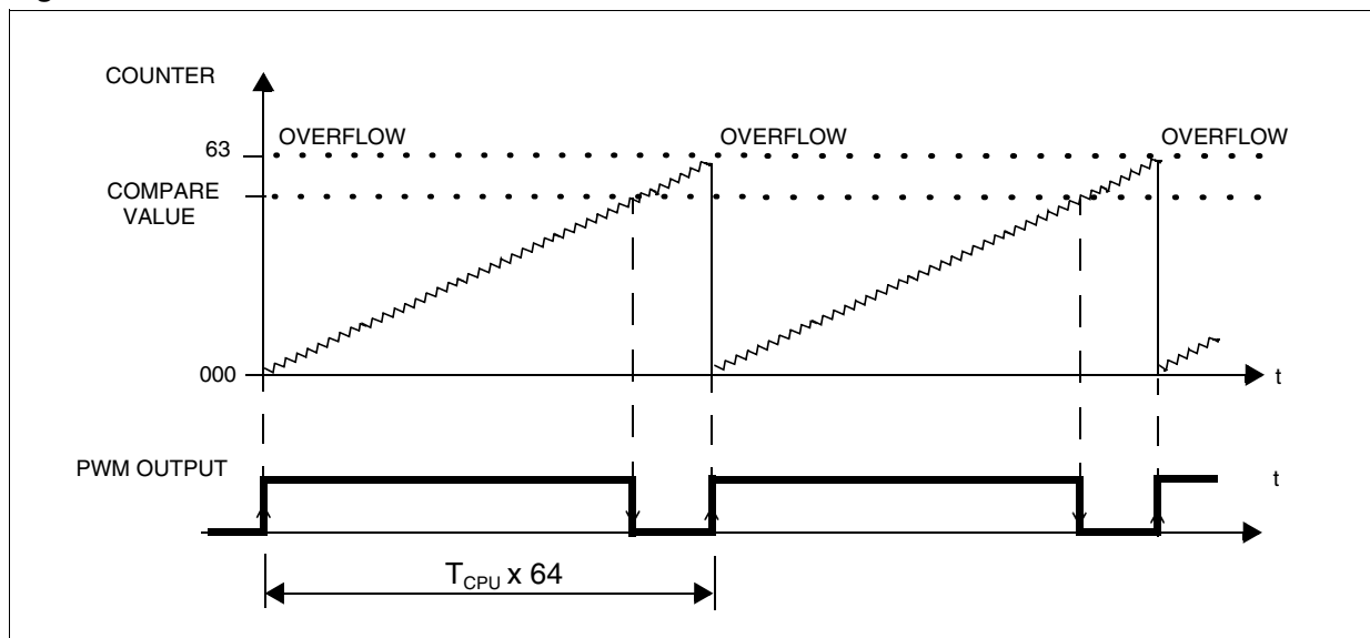
Figure 48. PWM Generation
