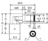
"E" type: (4.2x6.0x10.0 CPØ1.4)
