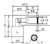
"D" type: (3.0 x 6.3 x 9)
