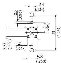
Hole pattern on PCB
