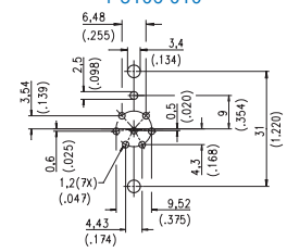
Hole pattern on PCB
