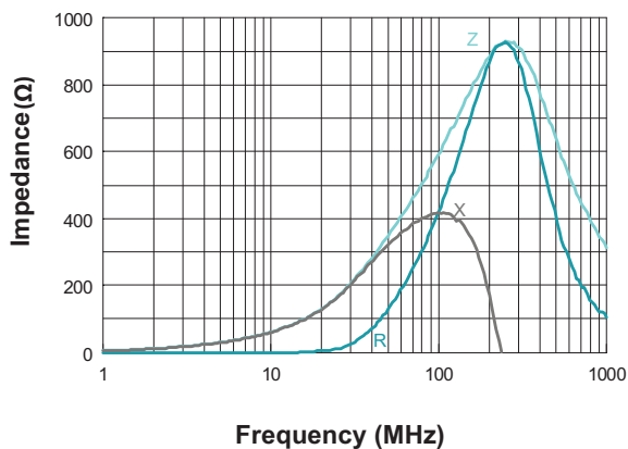
PE-1206FBA601ST
