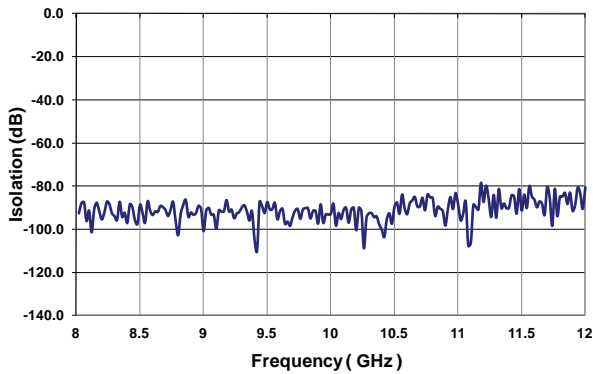
Isolation (8-12 GHz)
