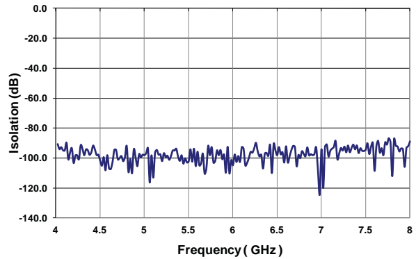
Isolation (4-8 GHz)
