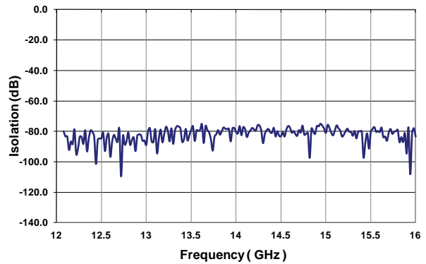
Isolation (12-16 GHz)
