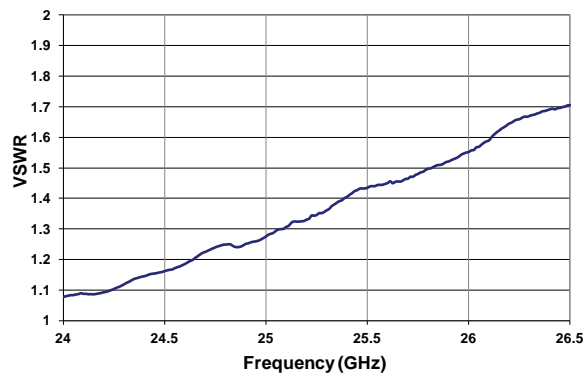
VSWR ( 24-26.5 GHz )
