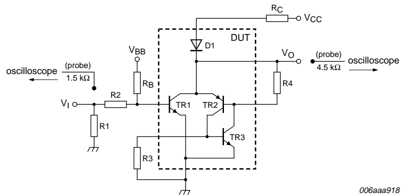
I_C = 0.05\text{ A} ; I_{B(on)} = 2.5\text{ mA} ; I_{B(off)} = -2.5\text{ mA} ; R_1 = 50\ \Omega ; R_2 = 1\text{ k}\Omega ; R_3 = 1\text{ k}\Omega ; R_4 = 1\text{ k}\Omega ; R_B = 1.5\text{ k}\Omega ; R_C = 150\ \Omega
