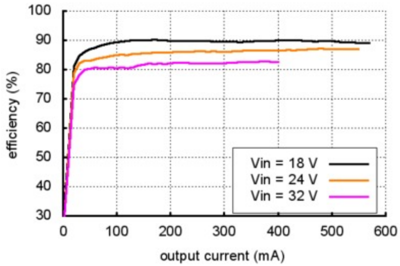
Pololu D24V6AHV Regulator Efficiency, Vout = 12 V
