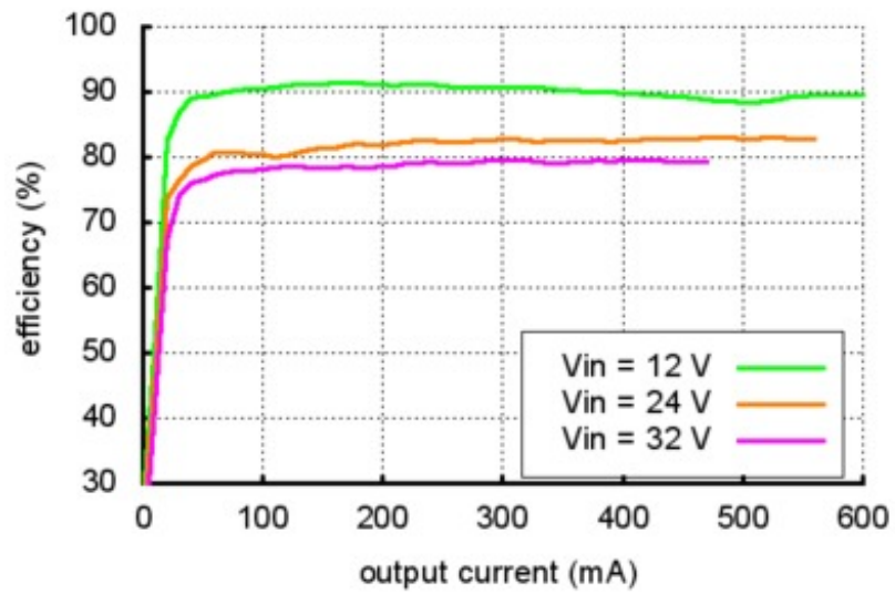
Pololu D24V6AHV Regulator Efficiency, Vout = 9 V
