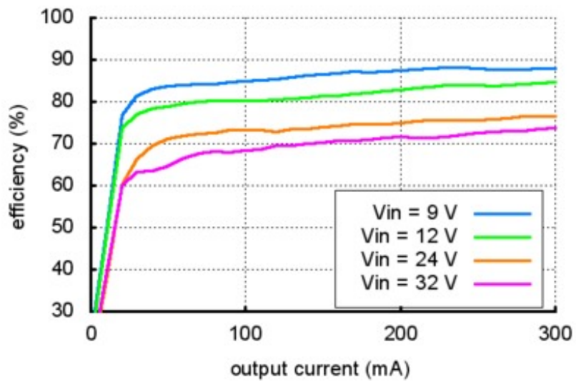
Pololu D24V3Axx Regulator Efficiency, Vout = 5 V
