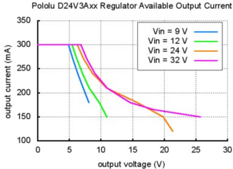
Typical available output current of Pololu step-down voltage regulator D24V3Axx.
