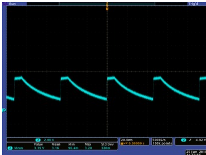
VOUT of the Pololu step-down regulator D24V3ALV when VIN is 5 V and the output voltage setting is higher than 5 V.
