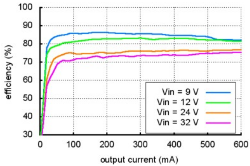
Pololu D24V6Axx Regulator Efficiency, Vout = 5 V
