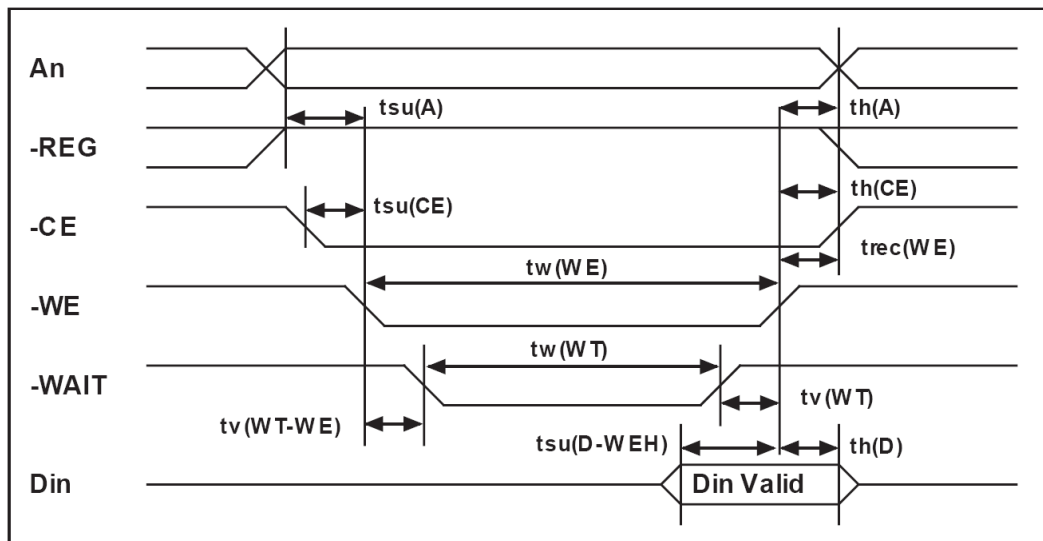
Common Memory Write Timing
