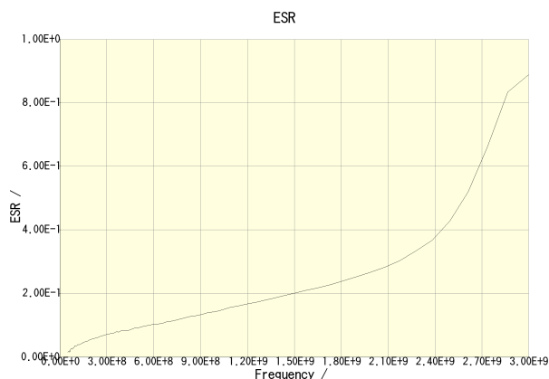
CGA2B2C0G1H470J050BA
