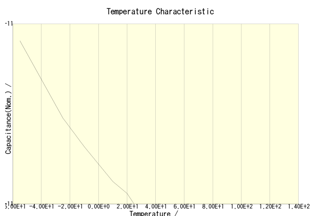
CGA2B2C0G1H470J050BA(DC Bias = 0V) CGA2B2C0G1H470J050BA(DC Bias = 25V)
