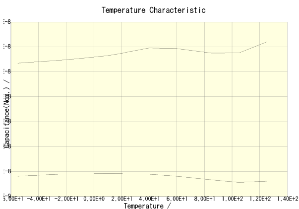
CGA4J3X7R2E223K125AA(DC Bias = 0V) CGA4J3X7R2E223K125AA(DC Bias = 125V)
