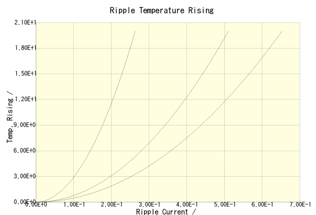
CGA4J3X7R2E223K125AA(100kHz) CGA4J3X7R2E223K125AA(500kHz) CGA4J3X7R2E223K125AA(1MHz)
