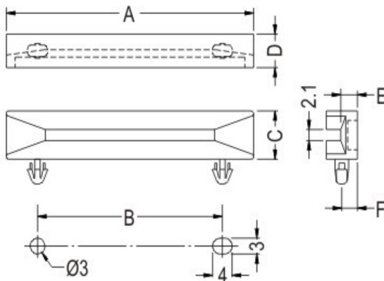
MOUNTING HOLES
