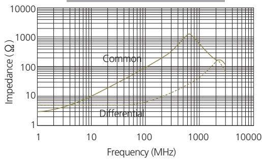
Impedance vs. Frequency Characteristics(Typ.)
