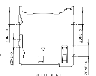
SHIELD PLATE
