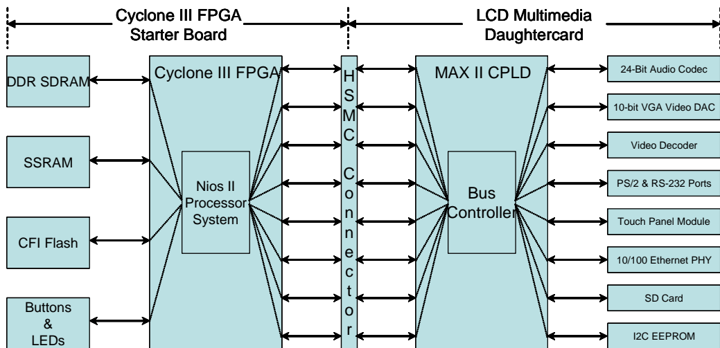
Figure 3-1. Block Diagram of Nios II Embedded Evaluation Kit, Cyclone III Edition
