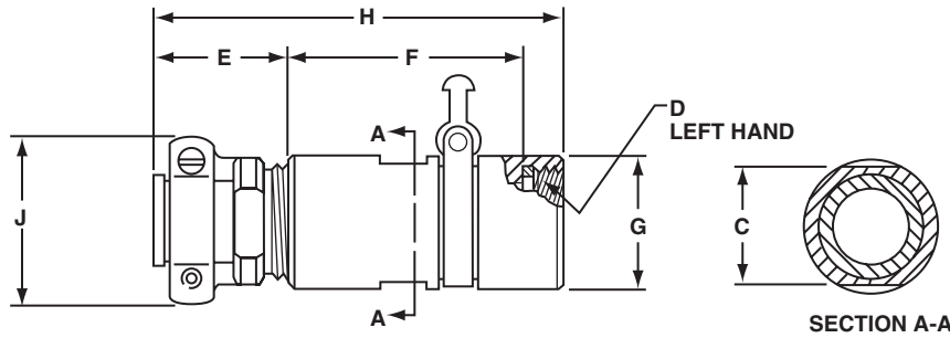
SECTION A-A Type I Straight
