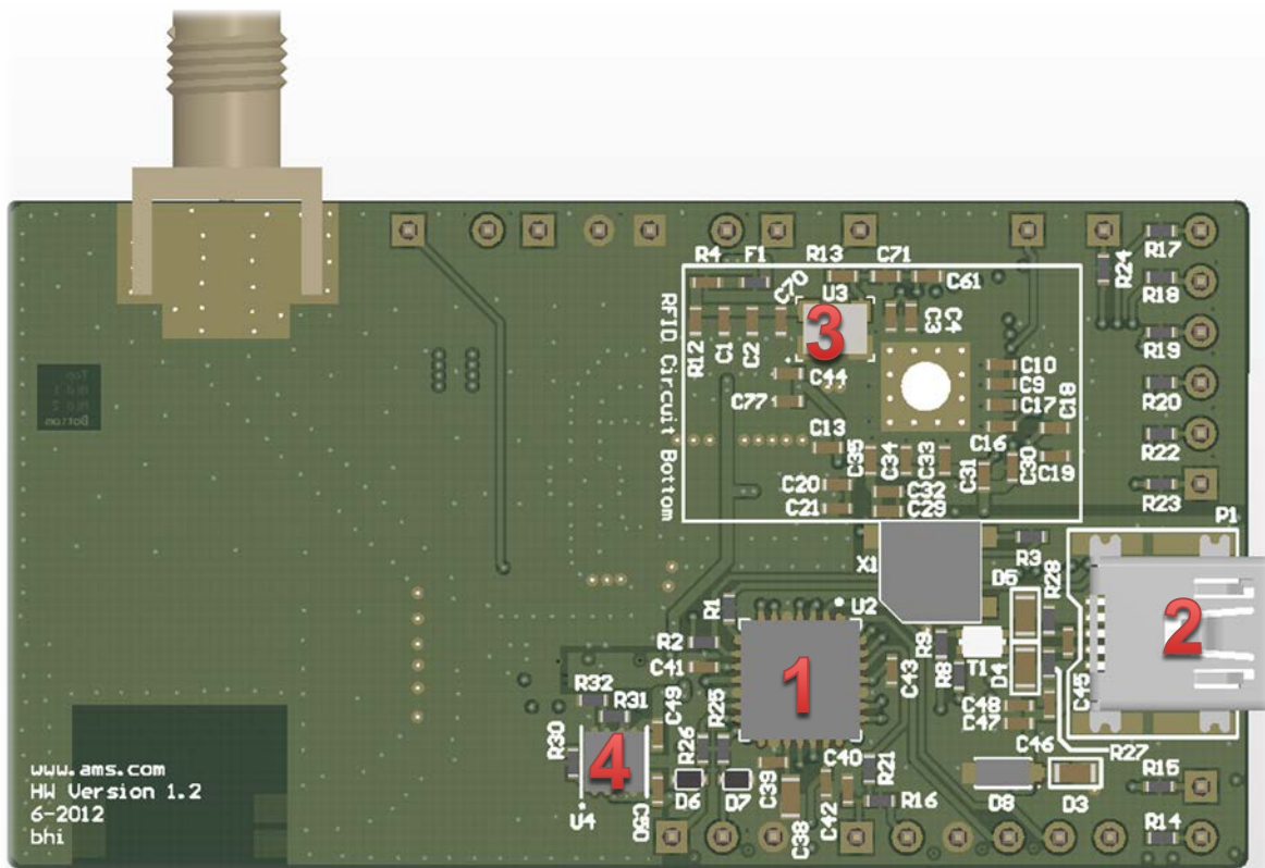
Figure 2 – Reader Bottom
