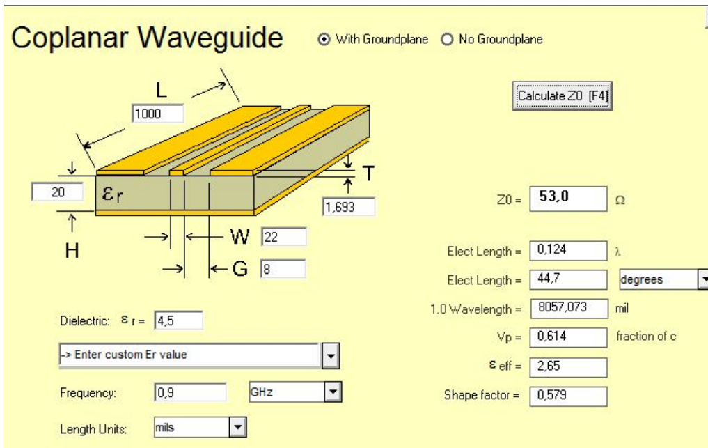
Figure 8 - RF Tracks - Impedance Calculation (dimensions in mil)
