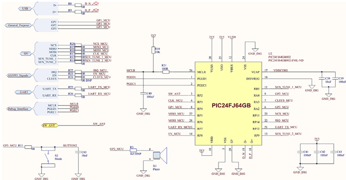
Figure 14 - Schematic Controller Section
