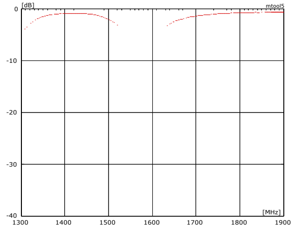
Reference Board A10137-D
