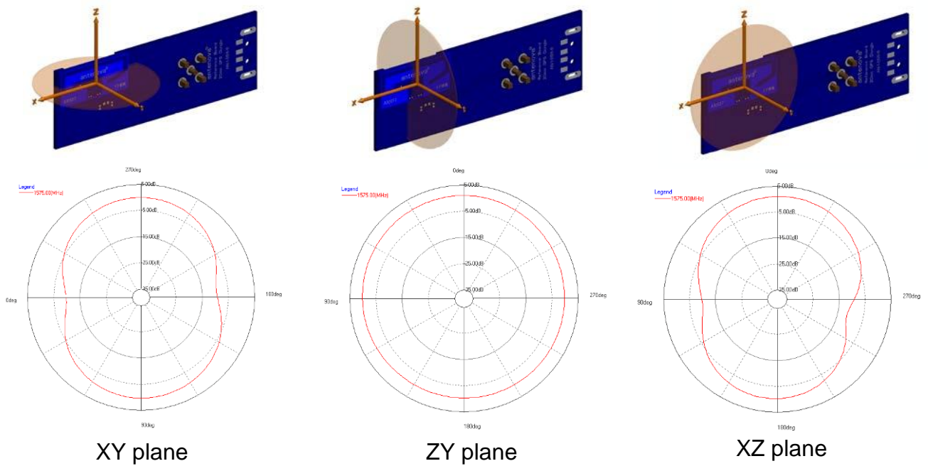
Patterns show combined polarisations measured on reference board A10137-D
