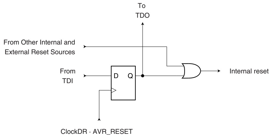
Figure 22-2. Reset Register
