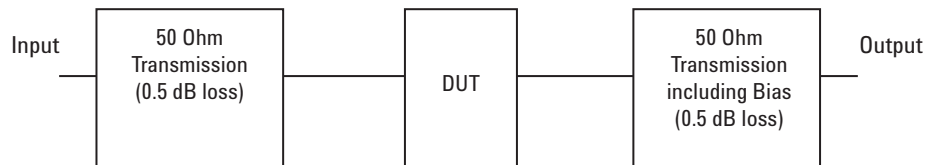
Block diagram of 900 MHz production test board used for V_d , Gain, P_{1\text{dB}} , \text{OIP}_3 , and NF measurements. Circuit losses have been de-embedded from actual measurements.
