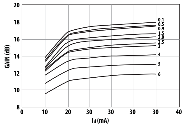
Figure 12. Gain vs. I d and Frequency (GHz).
