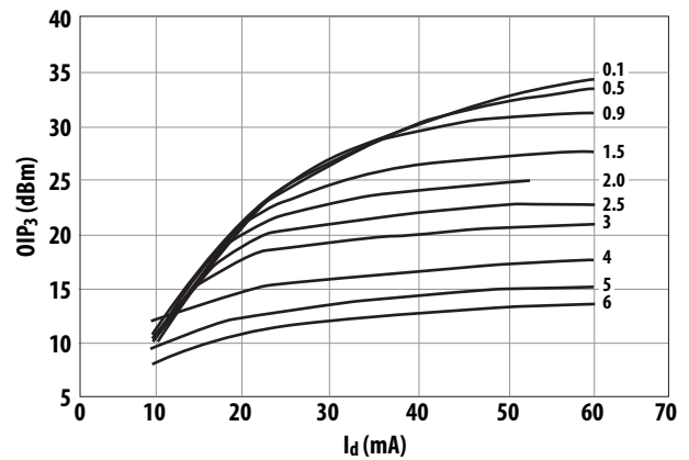
Figure 14. OIP 3 vs. I d and Frequency (GHz).
