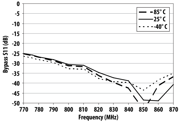
Figure 17. Bypass S11 vs Frequency
