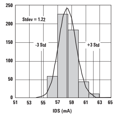
Figure 3. IDS; LSL = 51 mA, Nominal = 58 mA, USL = 65 mA.
