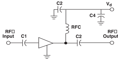
Figure 15. Schematic Diagram.
