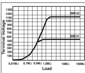
Terminal Characteristics
