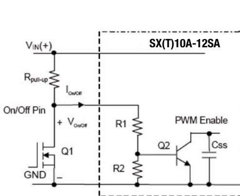
Fig. 23 Circuit Configuration for using Negative Logic On/Off
