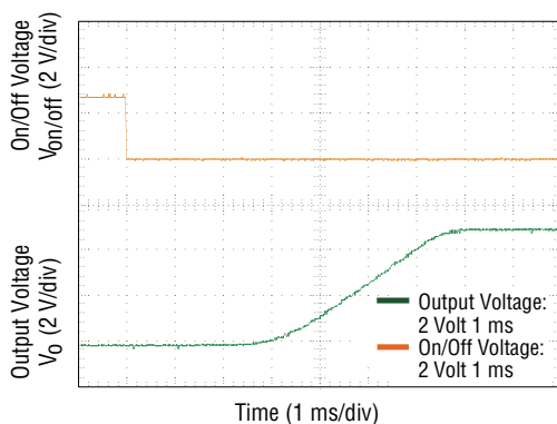
Fig. 15 Typical Start-up using Negative Remote On/Off with Low-ESR External Capacitors (10x100 \mu F Polymer) ( V_{in} = 12 V_{dc} , V_o = 5.0 V_{dc} , I_o = 10.0 A , C_o = 1000 \mu F )
