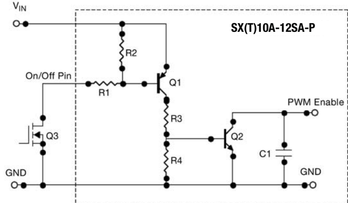
Fig. 24 Circuit Configuration for using Positive On/Off
