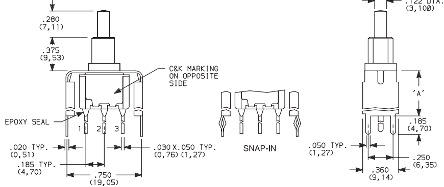
8161SH9_BE2 SPDT
