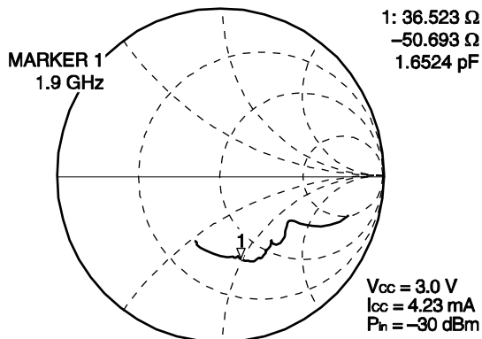
S11-FREQUENCY
