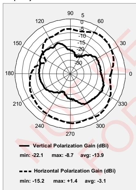
Frequency = 2480 MHz
