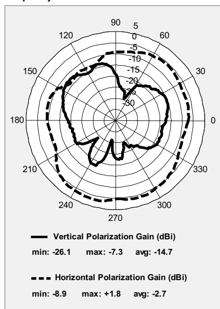
Frequency = 2405 MHz
