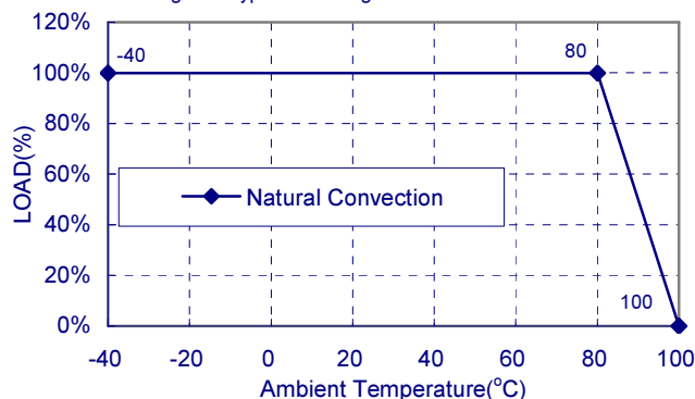
Figure1. Typical Derating curve for Natural Convection
