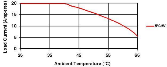
Derating Curve: DC60A10
