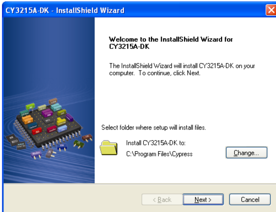
Figure 2-3. InstallShield Wizard
