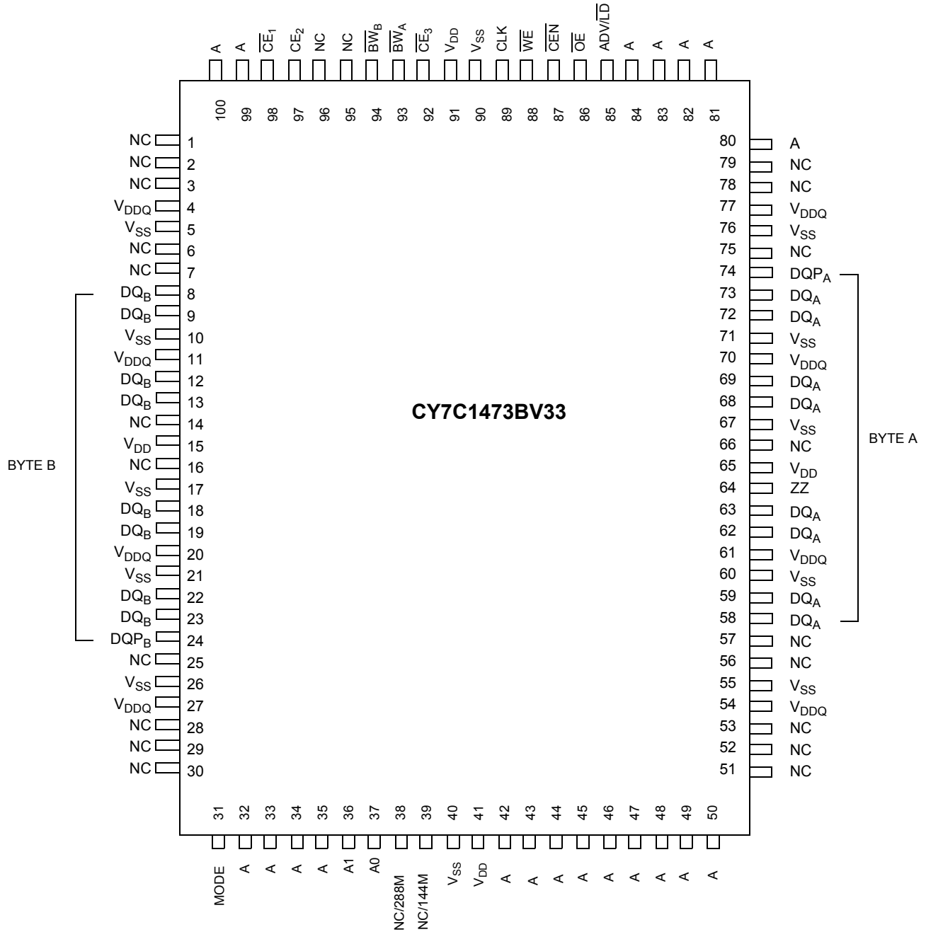
CY7C1473BV33 (4 M × 18)
