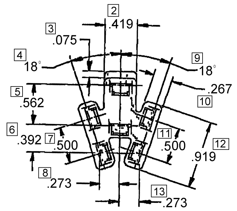
MATING END
