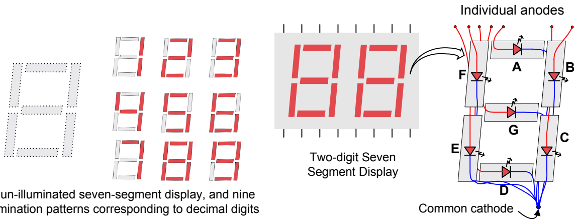
Fig. 14. Seven-segment displays.
