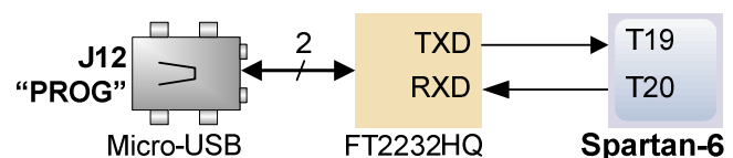
Fig. 8. UART interface.
