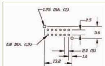
P.C. MOUNTING
