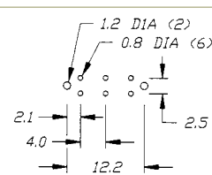
P.C. MOUNTING
