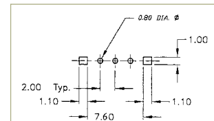
P.C. MOUNTING
