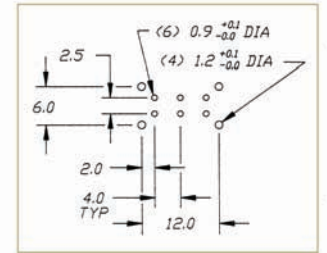
P.C. MOUNTING
