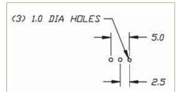
P.C. MOUNTING
