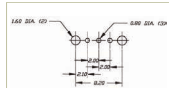
P.C. MOUNTING
