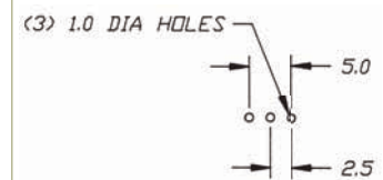
P.C. MOUNTING
