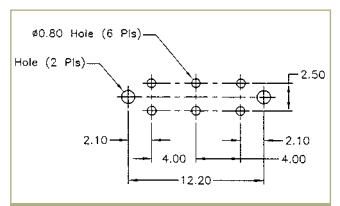
P.C. MOUNTING
