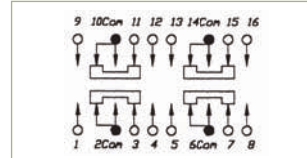
SCHEMATIC
