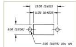
PANEL MOUNT
