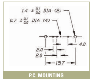
P.C. MOUNTING
