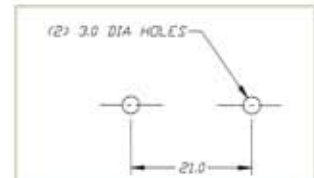
PANEL MOUNT
