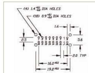
P.C. MOUNTING
