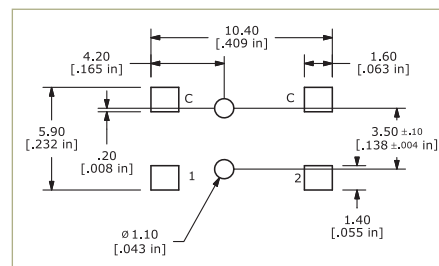
P.C. MOUNTING
