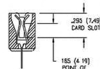
SECTION THROUGH CONTACT POSITION
