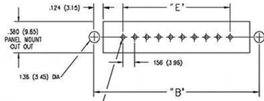
CONNECTOR MOUNTING PATTERN
