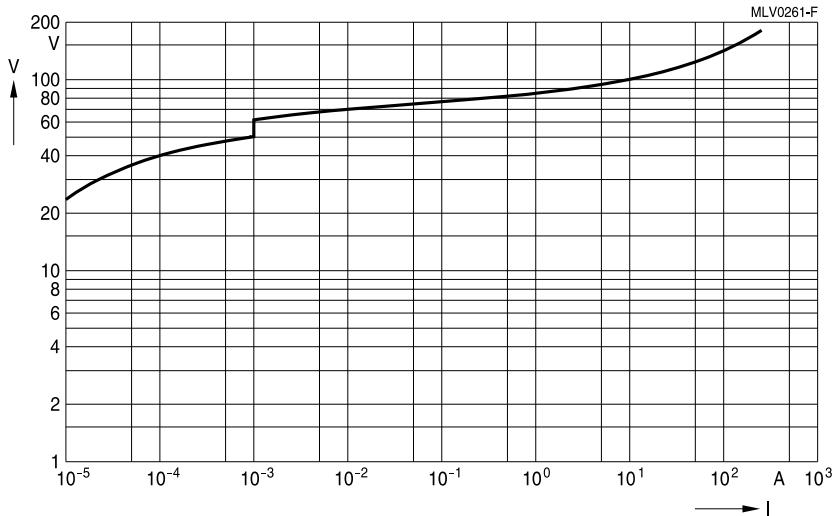
CT1210K35G
