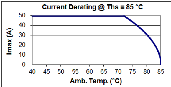
B25620B0227K881/B25620C0227K881
