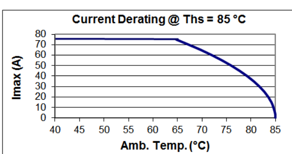
B25620B1427K101
