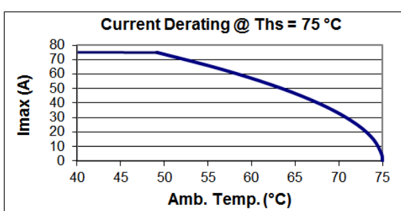
B25620B1457K103
