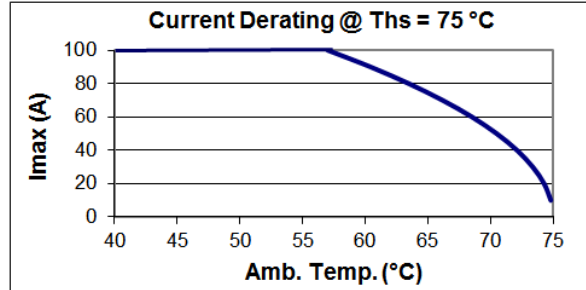
B25620D1707K103
