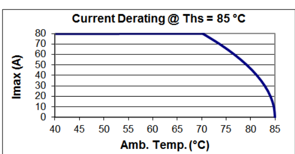
B25620D1457K101
