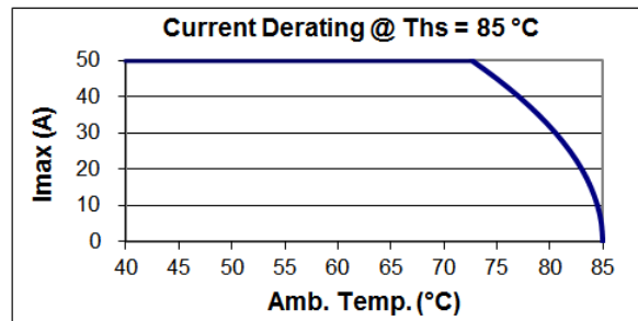
B25620B0357K881/B25620C0357K881
