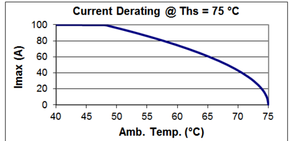
B25620B1118K103
