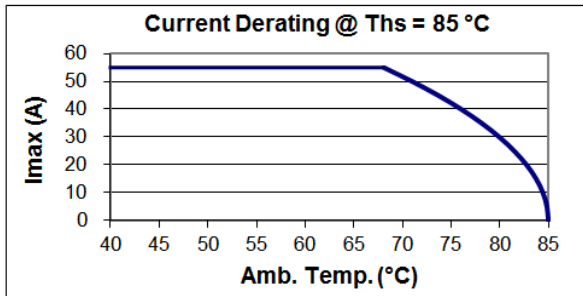
B25620B0707K701
