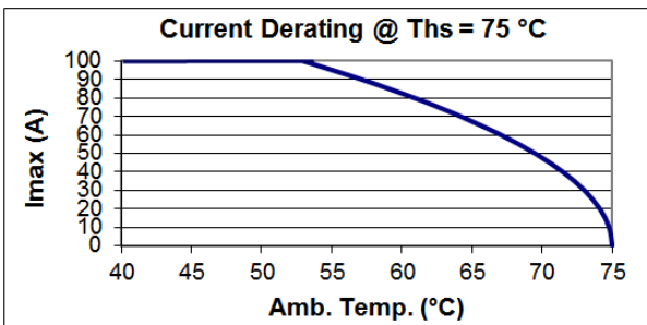
B25620B0158K883/B25620C0158K883
