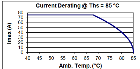
B25623B0837K904
