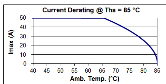
B25620B0557K881/B25620C0557K881
