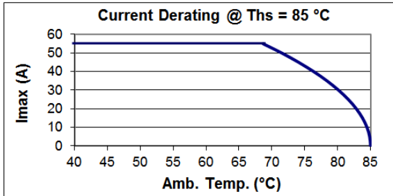
B25623B1277K104
