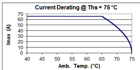
B25620B0447K883
