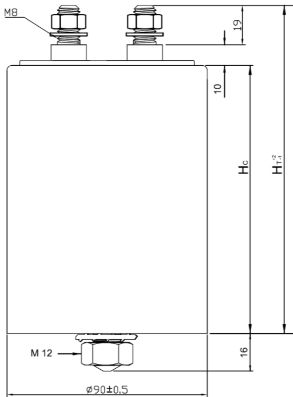
Figure 3: - B25623B - Ø 90 mm - Male terminals (M8) - Between terminals 45±0.5 mm
