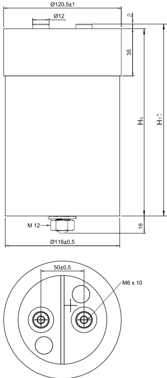
Figure 5: - B25620C / B25620D - Ø 116 mm - Female terminals (M6) - Between terminals 50±0.5 mm
