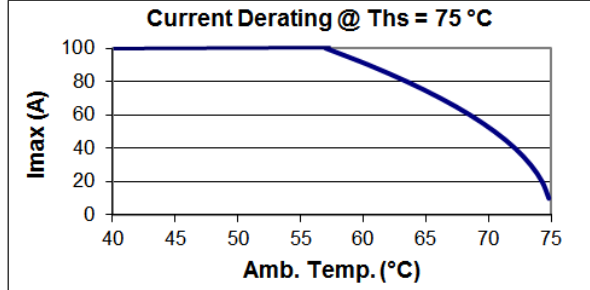
B25620D1707K103
