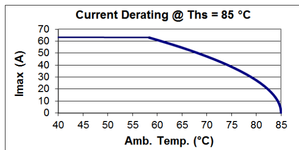
B25620B1427A101
