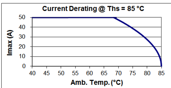
B25620B1317K101
