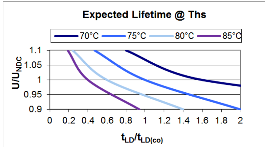
Service life t_{LD} at different hotspot temperature ( \Theta_{hs} ) and voltage V
