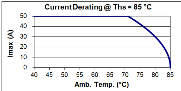
B25620B1147K101
