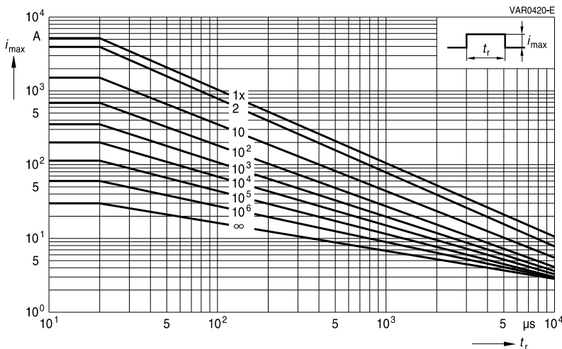
SIOV-S14K385 ... K680E2
