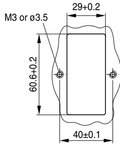
Mounting holes for Mounting version I
