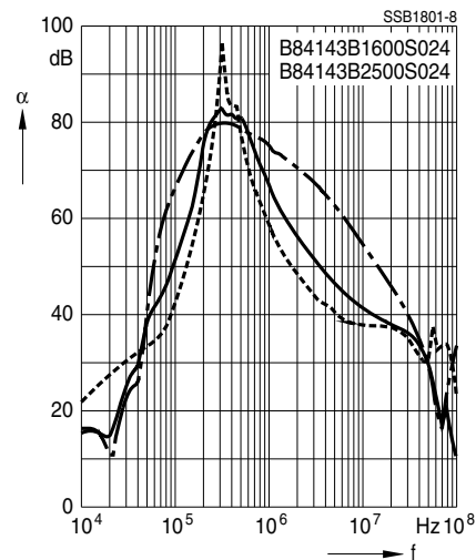
Filters for 1600 and 2500 A (Type S024)
