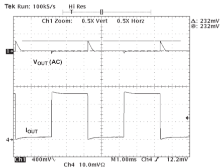
Fig. 8: Load Regulation, I_0=100\mu A \sim 500mA
