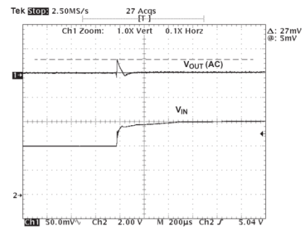
Fig. 9: Regulation, Line Step from 4V to 6V, I_0=1mA
